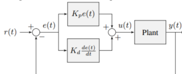
Gambar 13 Diagram Blok Kendali Proportional-Derivative
